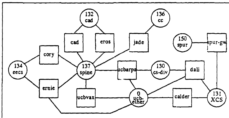
FIGURE 2-1. UCB NETWORKS AND GATEWAYS
