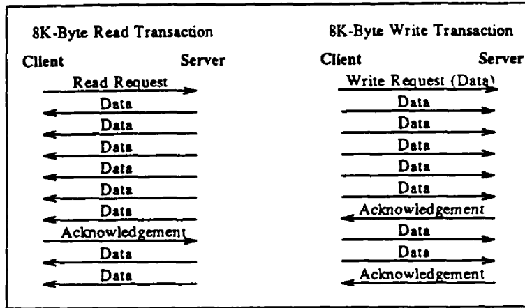
FIGURE 6-5. NETWORK DISK PROTOCOL TRANSACTIONS
